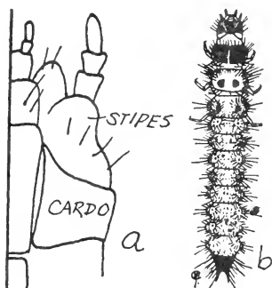
Fig. 246. a, Ventral half of the head; b, Callimerus arcifer Chapin.
